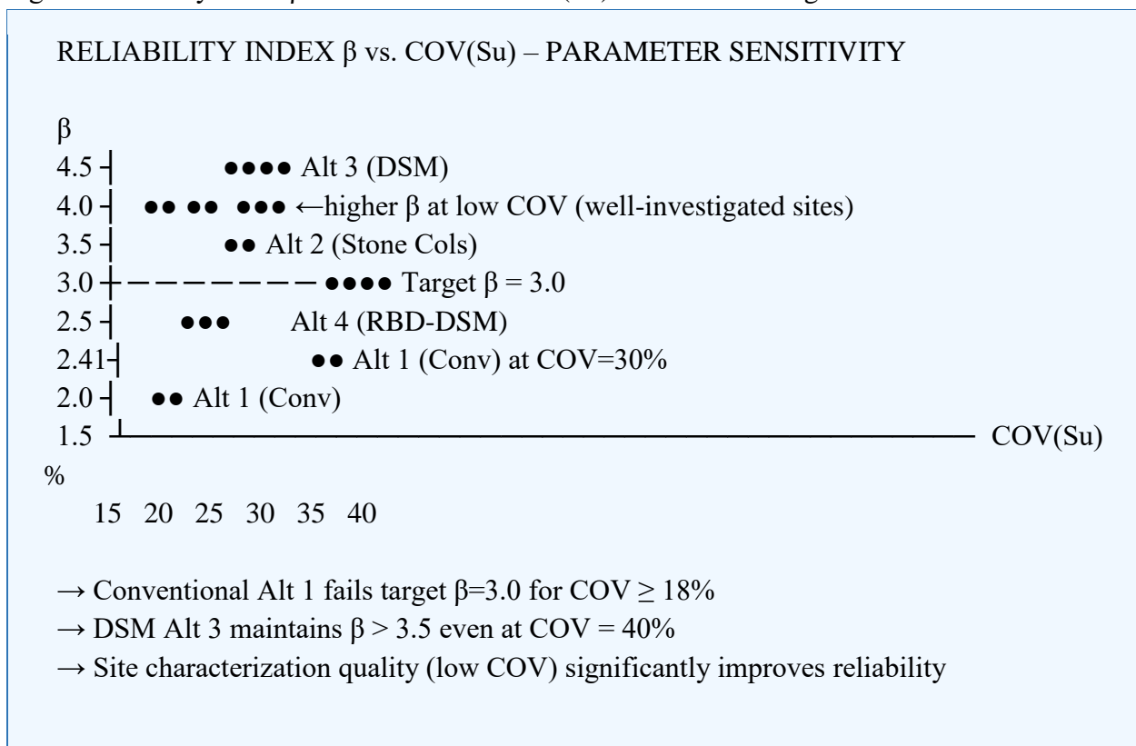
Fig. 2. Reliability index \beta as a function of COV(S_u) for the four design alternatives
